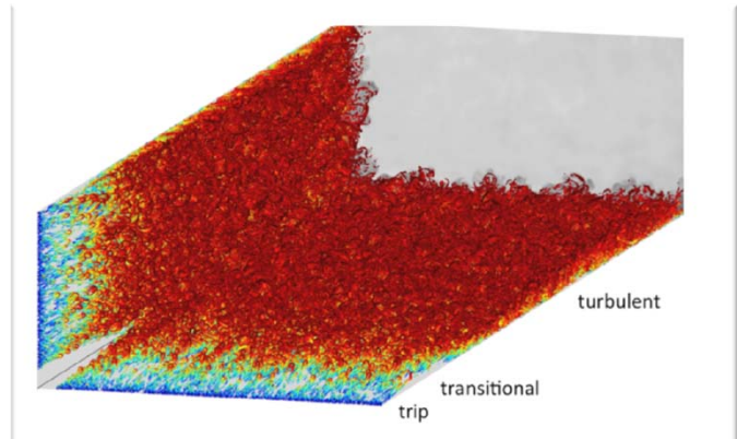
1 st place video 2014 "Large Eddy Simulation of Mach 2.25 flow in a 2:1 duct" Nicholas Bisek, AFRL
