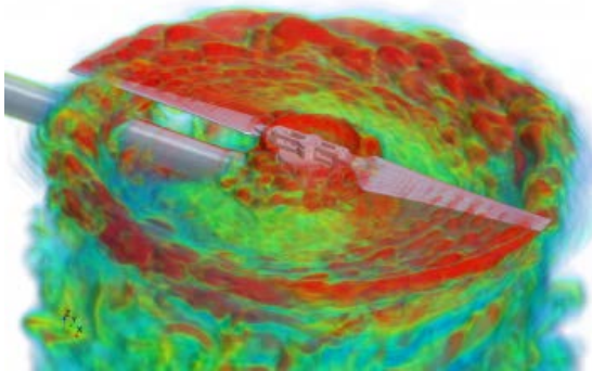
1 st place photo 2018 “Vortices Shedding from a drone rotor” Zhenyu Wang (OSU)
