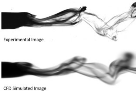
Dye Injection into Turbulent Water
